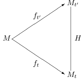
Figure 1: Homotopic Models
